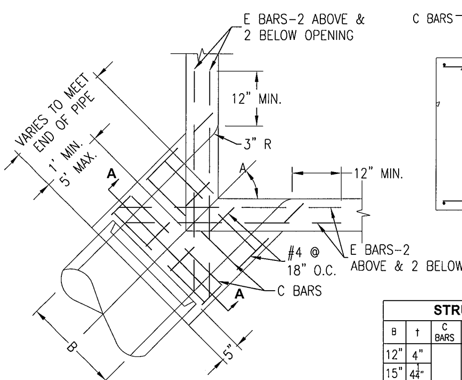
PLAN CORNER CONNECTION
