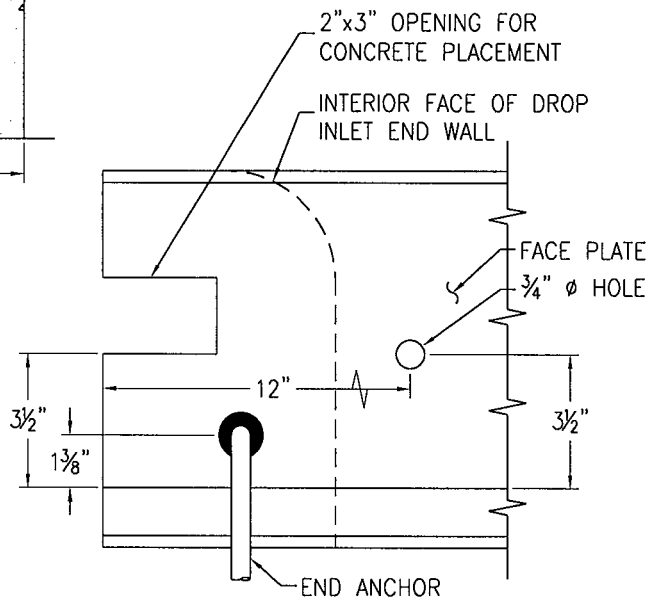
END DETAIL
