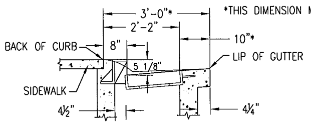
SECTION A-A TYPE 1A-ROLLED C&G
