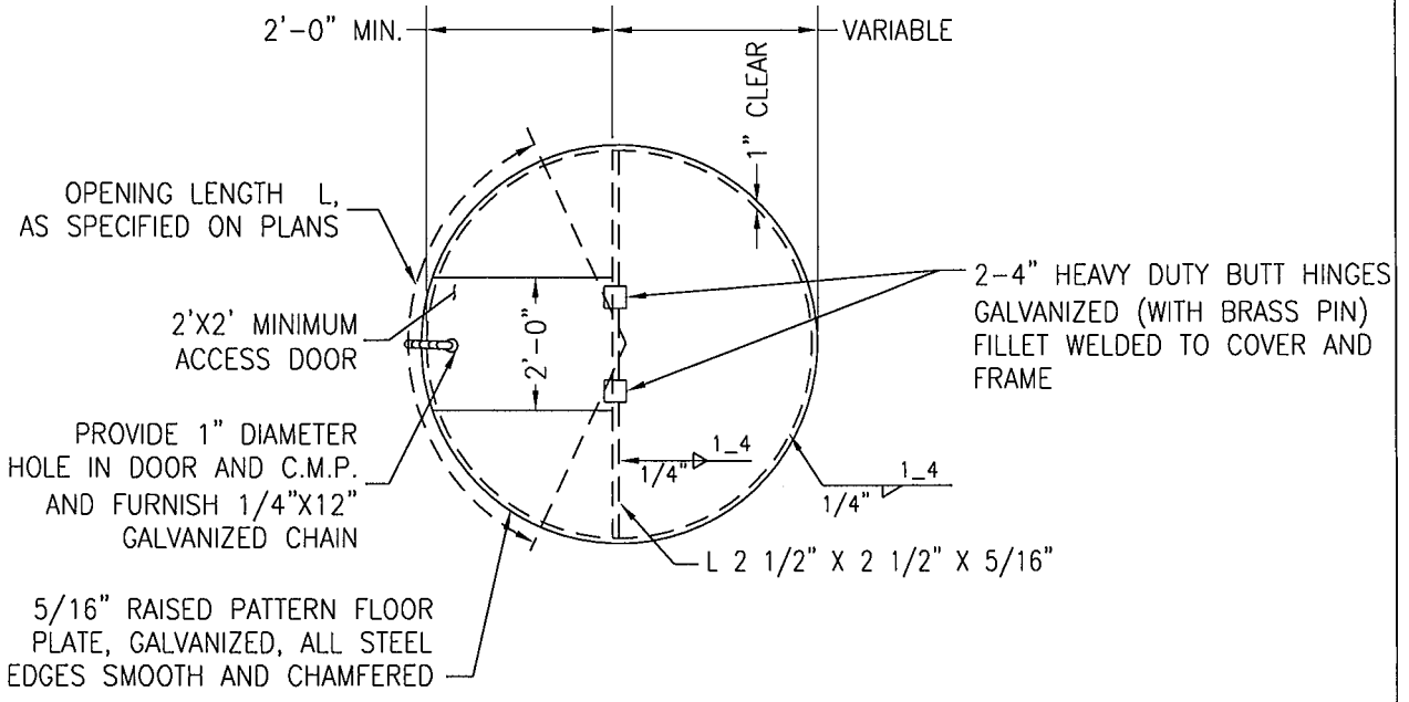
PLAN 42" DIAMETER TO 72" DIAMETER C.M.P. INLET
