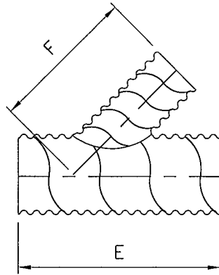
WYE LATERAL
