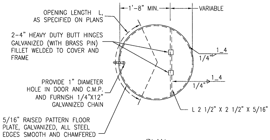
PLAN 24" DIAMETER TO 36" DIAMETER C.M.P. INLET
