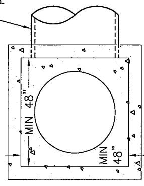
BOX BASE (PLAN VIEW)
