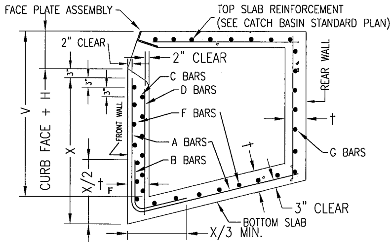
TYPICAL REINFORCEMENT DETAILS
