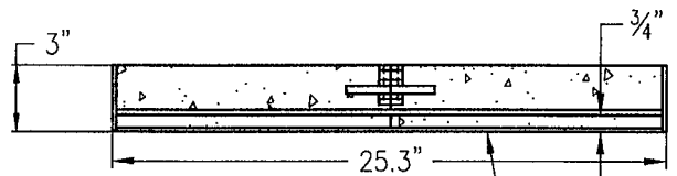
SECTION 3/16" FRAME
