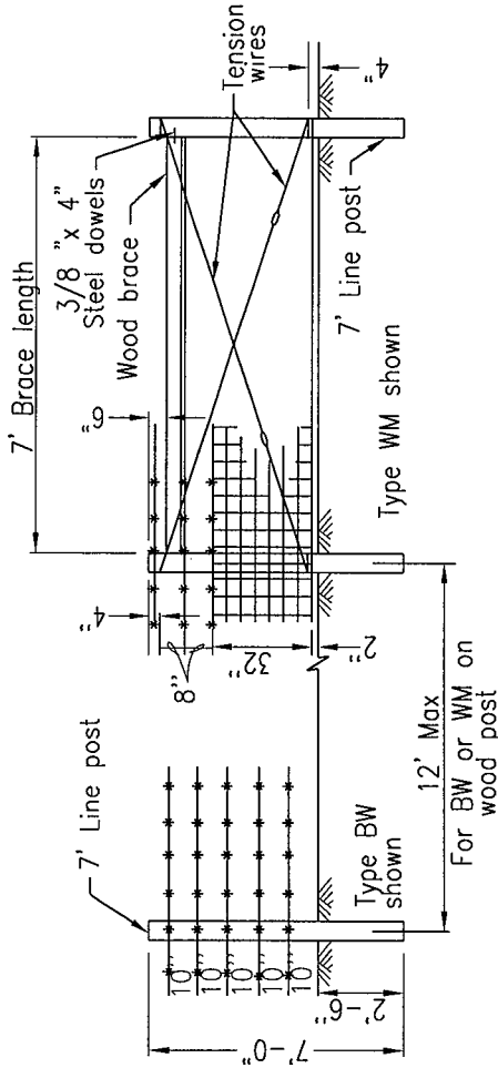
PULL POST ASSEMBLY
