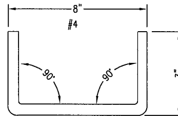
DOWEL DETAIL
