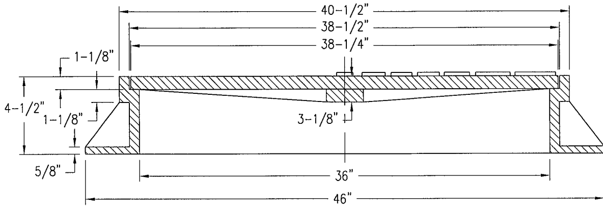
SECTION C-C
