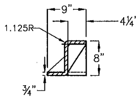
SECTION C-C OPEN-BACK HOOD
